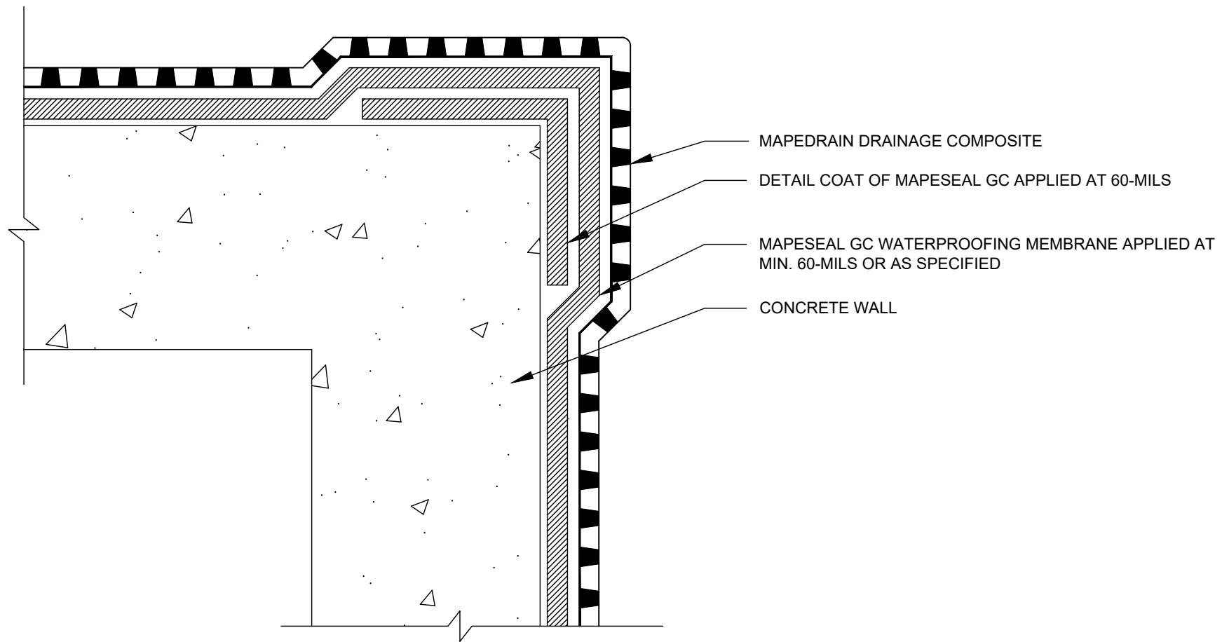
PLAN VIEW
